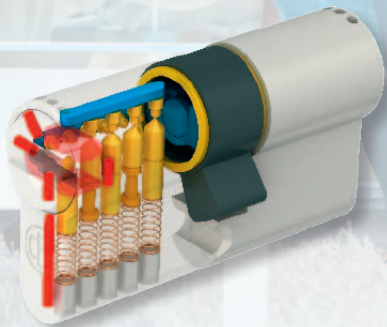
Security cylinder 910 WR
